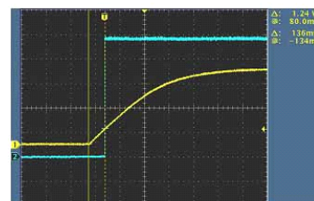
CH1: Von/off CH2: Vo Delay time: 136mS
