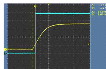
CH1: Von/off CH2: Vo Delay time: 64mS
